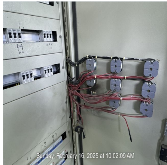
Electrical box/cabinet with wiring
